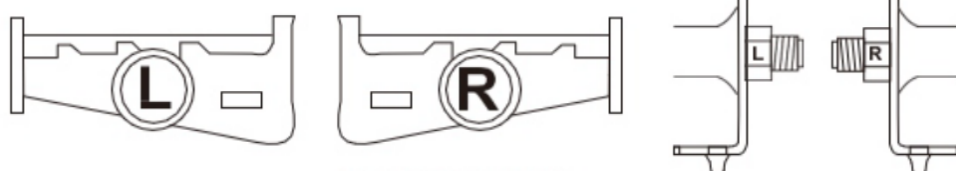
fig. 11 Attaching pedals
